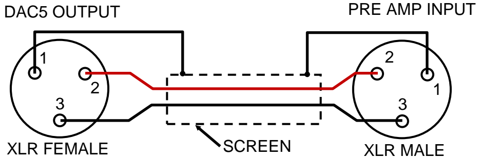
CONVENTIONAL: SCREEN CONNECTED AT BOTH ENDS
