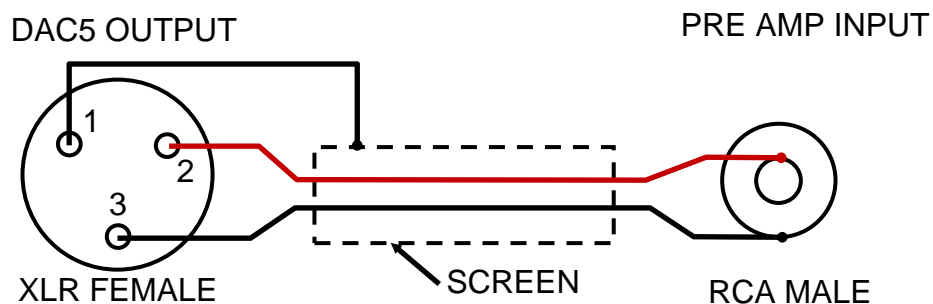
CABLE CONFIGURATION FOR XLR BALANCED OUTPUT TO RCA UNBALANCED INPUT
