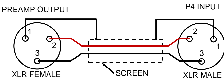
CONVENTIONAL: SCREEN CONNECTED AT BOTH ENDS
