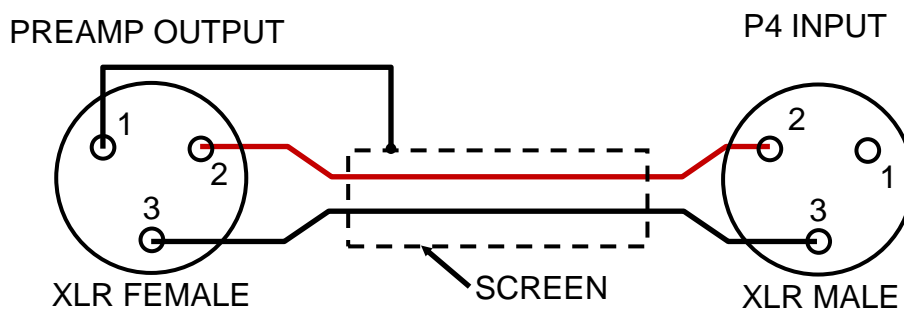
SCREEN CONNECTED AT PREAMP END ONLY, TO ELIMINATE GROUND LOOPS
