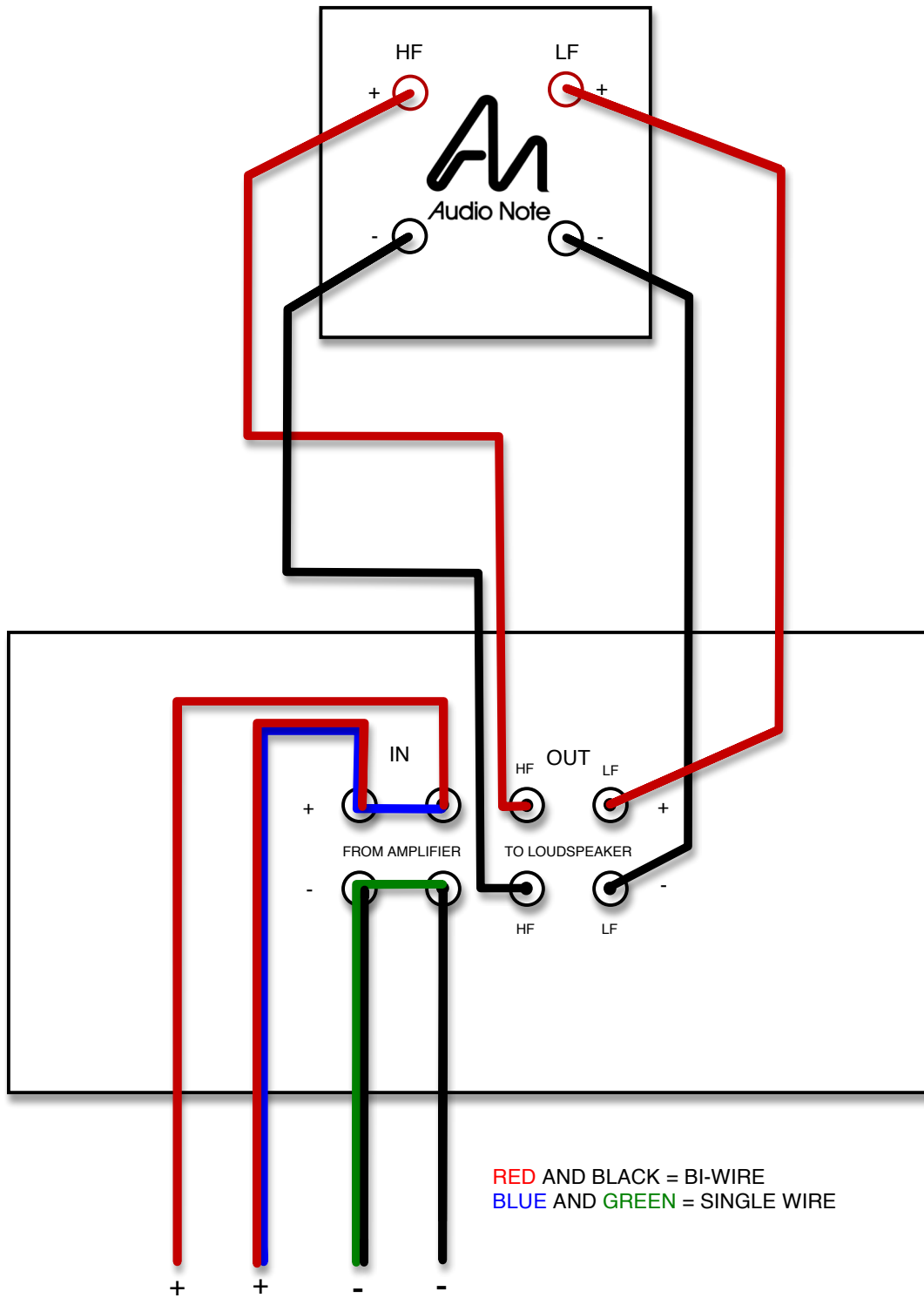
LOUDSPEAKER CONNECTIONS FROM AMPLIFIER
