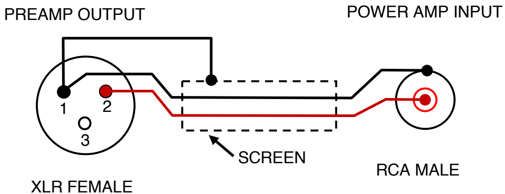
CABLE CONFIGURATION FOR XLR BALANCED PREAMP OUTPUT TO RCA UNBALANCED AMPLIFIER INPUT
